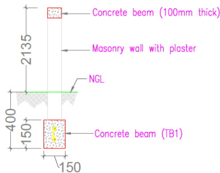
wall detail
